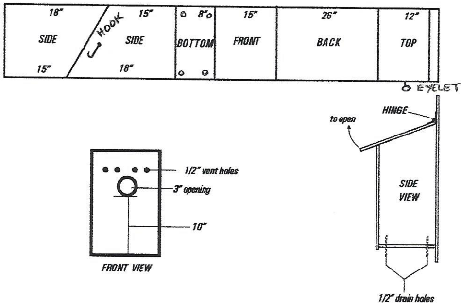
Plank 1" x 10" x 8' cut diagram
